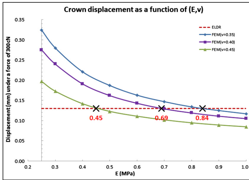
Fig 4. Crown displacement as a function of (E, v), with E from 0.25 to 1 MPa, under a 300-cN force.
