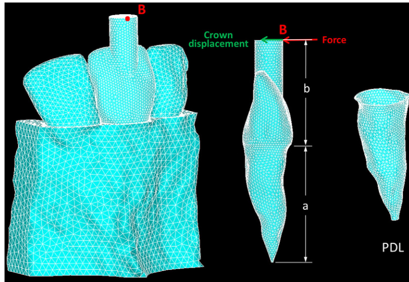
Fig 2. Finite element model of a 3-tooth periodontal ligament and bone complex.
