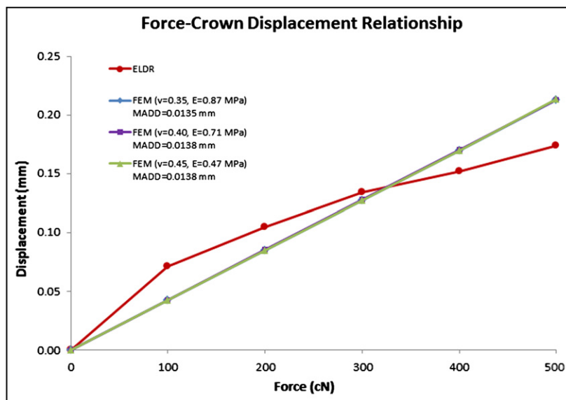
Fig 5. Crown-displacement relationships with minimal mean absolute displacement differences for the 3 best E and v pairs. The experimental load-displacement relationship is also shown.
