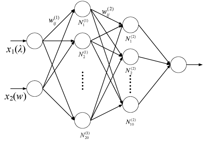
Fig. 11. The employed “2-20-10-1” BP neural network.
