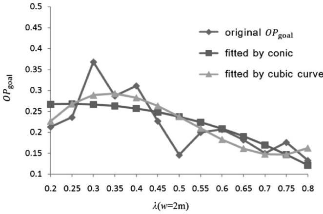
Fig. 10. OP_{\text{goal}} changes with \lambda and fitting by conic and cubic curves. The fitting errors by conic and cubic curves reach 1.101 and 0.079 separately.
