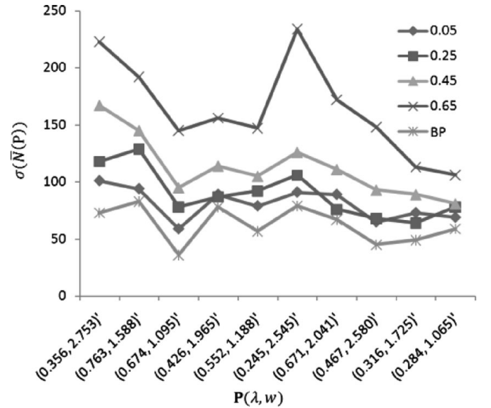
Fig. 15. Standard deviation of average sampling number of times with different values of P_{goal} .
