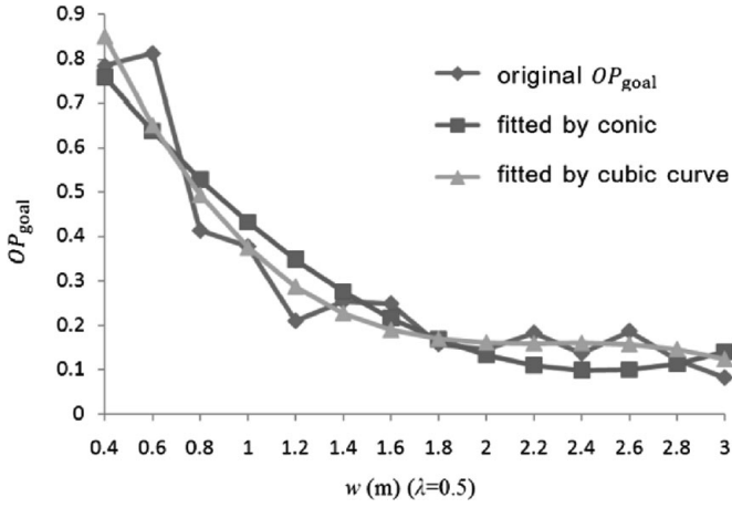
Fig. 9. OP_{\text{goal}} changes with w and fitting by conic and cubic curves. The fitting errors by conic and cubic curves reach 0.174 and 0.161 separately.
