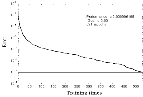
Fig. 12. The BP neural network converges after 531 trainings. The learning rate is 0.01, and the error limit is 0.001.
